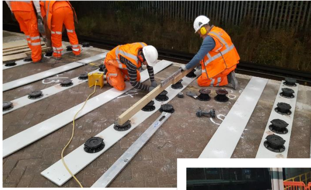
STAGE 2 SETTING PEDESTALS TO BACKFALL
