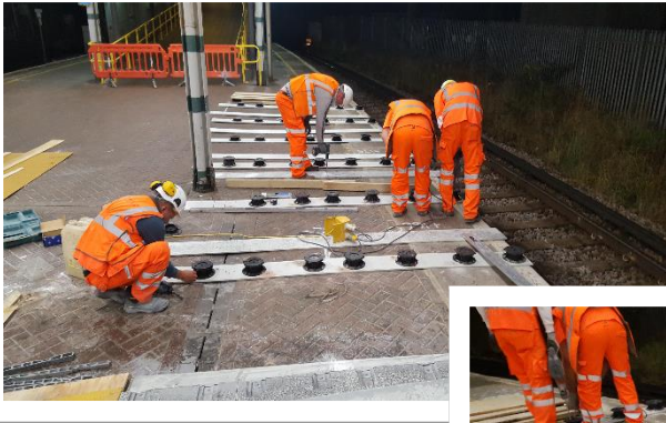
STAGE 1 LAYING PEDESTAL SUB FRAMES
